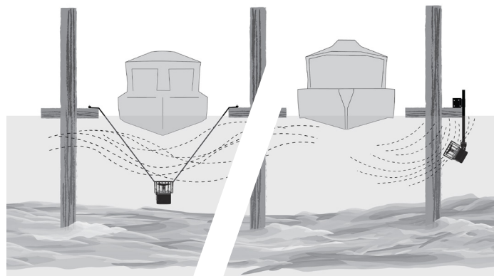
Vertical suspension
